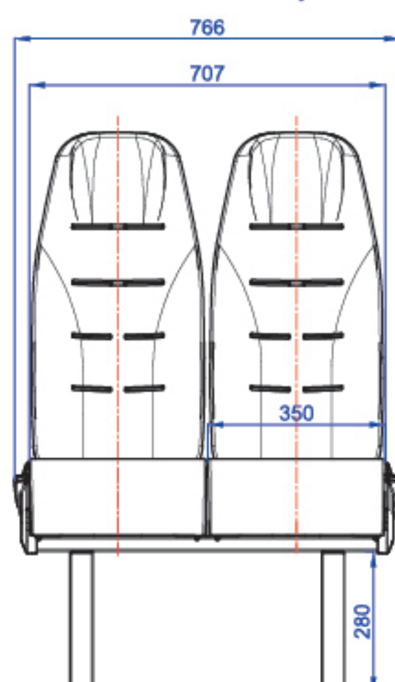
TECHNICAL DRAWING (FRONT VIEW)
